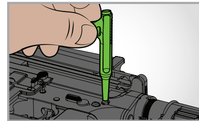
Use 3-in-1 tool to punch takedown pin
